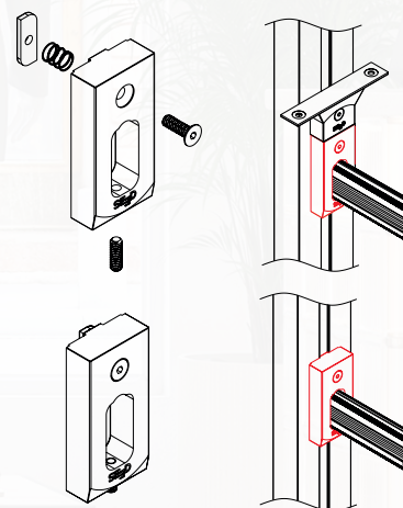
Wardrobe rail support assembly
