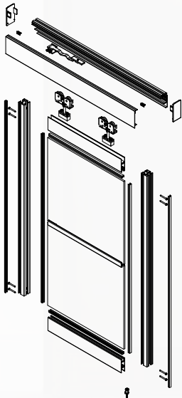
Suspended sliding door 70kg
