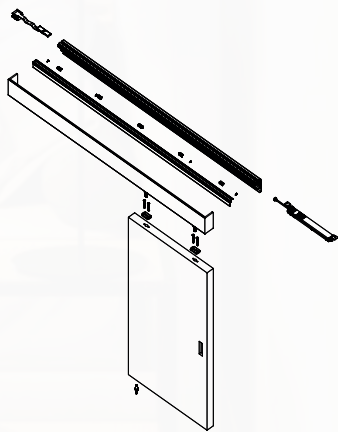
Suspended sliding wooden door 70kg
